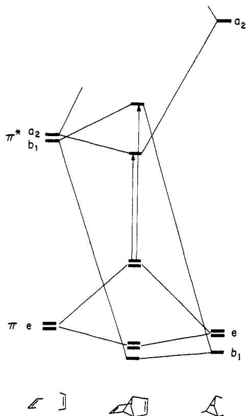
Figure 7. Interaction diagram for the mixing of ethylene orbitals (left) with cyclobutane orbitals (right) in tricycloocta[3.3.0.0 2,6 ]-octadiene. Note that the cyclobutane orbitals of Figure 4 have now been classified in D_{2d} symmetry. The arrows indicate allowed electronic transitions.
